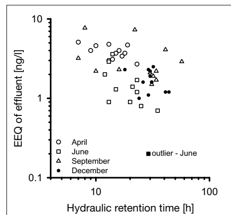
Fig. 5. Relationship between the hydraulic retention time (HRT) and the estrogenic activity (EEQ) of effluent over four 12-day sampling periods. The association between HRT and EEQ was negative in all but one sampling period (small filled circles). [20]
