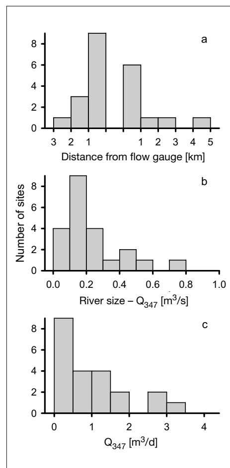
Fig. 7. Characteristics of sampling locations in Study IV. (a) Distance between the flow gauge and the effluent discharge. (b) Q_{347} , the flow exceeded on 347 days in a year, a measure of river size. (c) A measure of effluent dilution: the Q_{347} over the person equivalents (PE) discharging into the river.
