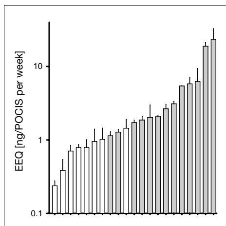
Fig. 8. Estrogenic activity (EEQ) sampled by POCIS [30] from 21 effluents. Open bars show STWs with a sand filter, grey bars show STWs without a sand filter. The standard error is derived from 2–3 POCIS.
