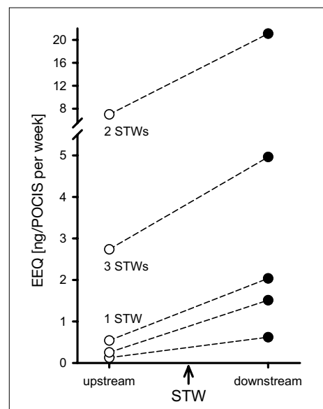
Fig. 6. Estrogenic activity (EEQ) accumulated by (POCIS [30] ) placed for 22 days up- (open circles) and downstream from sewage treatment work discharges (STW). [26] Lines connect the up- (open-circles) and downstream sampling sites (filled circles); Numbers in the graph denote the amount of discharges further upstream.
