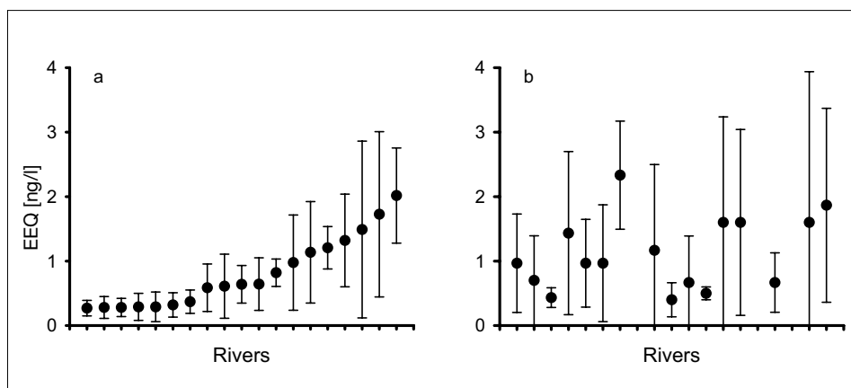
Fig. 2. (a) Average estrogenic activity (EEQ, ng/l; \pm standard deviation) of three grab samples collected from 19 rivers in winter downstream from a discharge of treated sewage effluent. Rivers are ordered in ascending average. (b) EEQ data from three samples taken in summer in 17 rivers, ordered as in panel (a). For presentation purposes – in order to keep the ‘winter’ and ‘summer’ y-axes to the same range – one summer data point is omitted ( 7.0 \pm 4.4 ng/l). [17]
